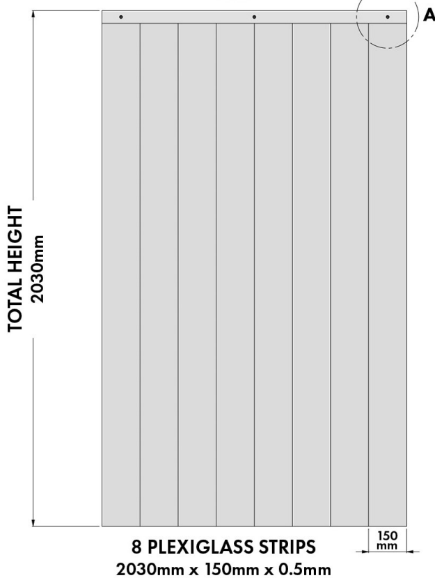
TEK SCREW SPACING 525mm
